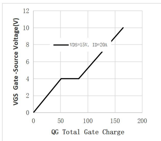
Fig.1 Gate-Charge Characteristics
