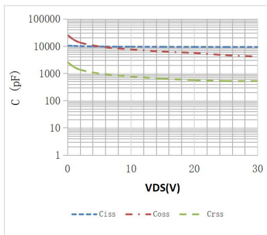
Fig.2 Capacitance Characteristics
